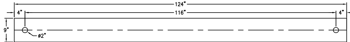
BASE PLATE ANCHOR HOLE DETAIL
