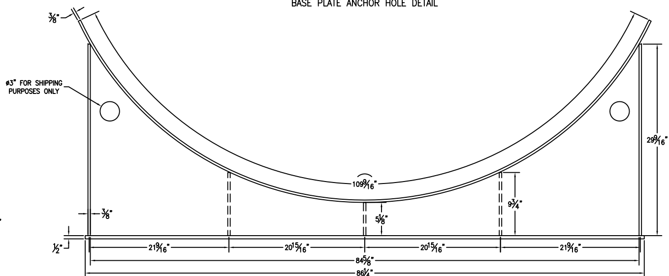
BASE PLATE ANCHOR HOLE DETAIL
