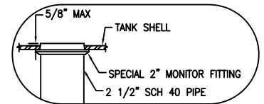
INTERSTITIAL MONITOR TUBE ASSEMBLY TOP
