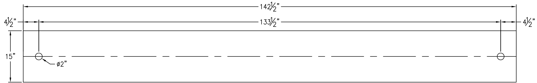
BASE PLATE ANCHOR HOLE DETAIL
